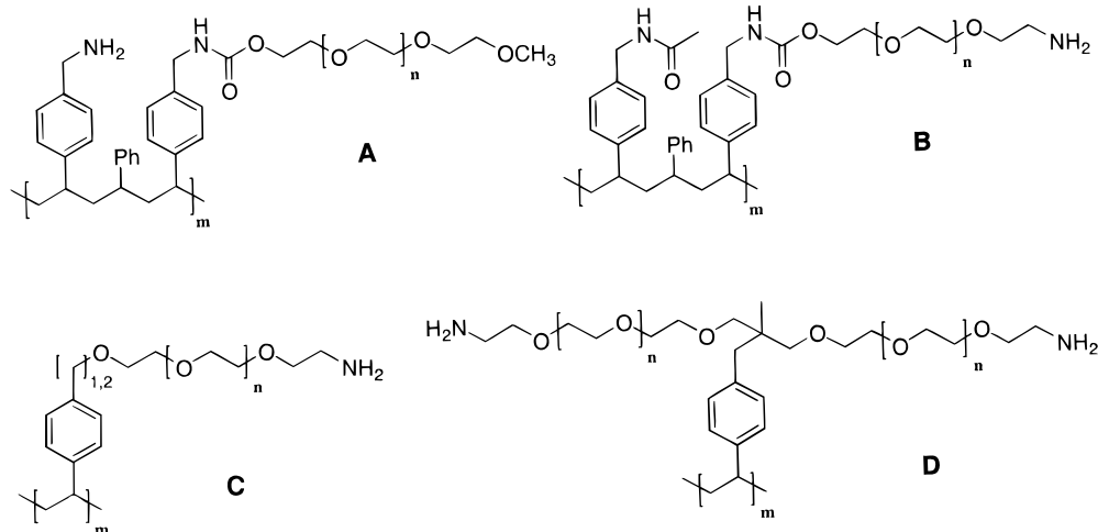
Figure 5. Structures of a variety of commercially available PS-PEG resins: (A) Champion I, NovaGel; (B) Champion II; (C) TentaGel (original formulation \text{CH}_2 PEG attachment, current TentaGel S formulation \text{CH}_2\text{CH}_2 attachment); (d) ArgoGel. All resins are shown in amino-functionalized forms.
